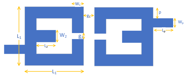
Fig. 1. SLR-based SOLR design and its parameters.
