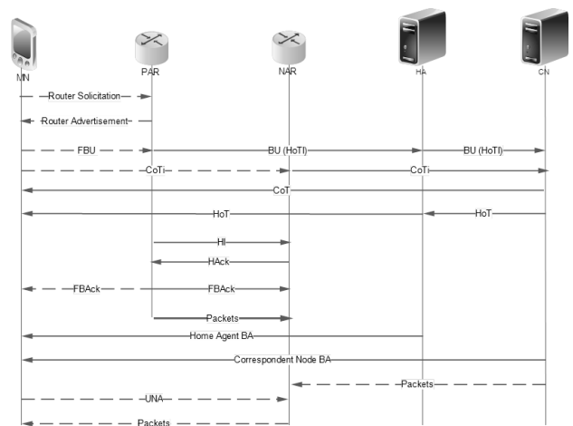
Fig.3 The Enhanced FMIPv6
