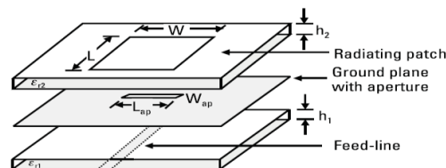
Fig. 1. Technique of Aperture Coupled Feed
