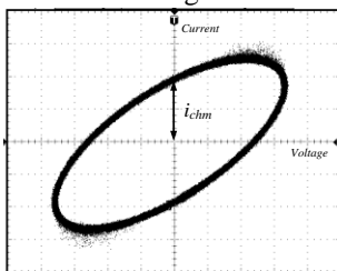
Figure 2. I-V characteristics in Lissajous Pattern
