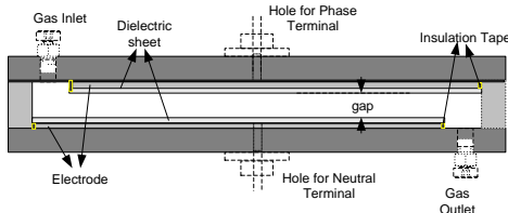
Figure 1. Ozone chamber
