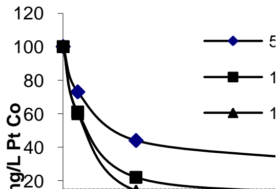
Figure 12. Colour removal as the function of dosage of ozone injection at different contact time
