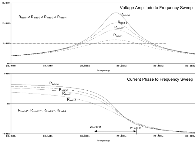
Figure 8 Simulation Result of Frequency Sweep Program
