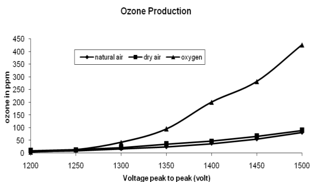
Figure 11. Ozone Concentration in ppm as a function of applied voltage in Volt
