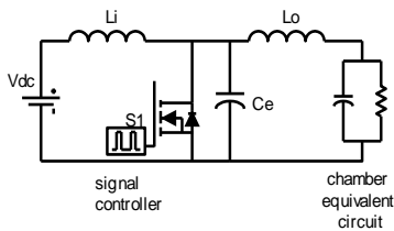
Figure 4. Fundamental Circuit of Single Switch Resonant Converter
