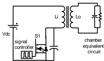
Figure 5. Single Switch Resonant Converter with step up transformer
