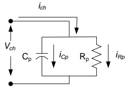
Figure 3. I-V Equivalent circuit of ozonizer
