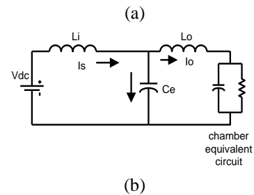
Figure 6. Single Switch Resonant Converter. (a) Switch turn on, (b) Switch turn off
