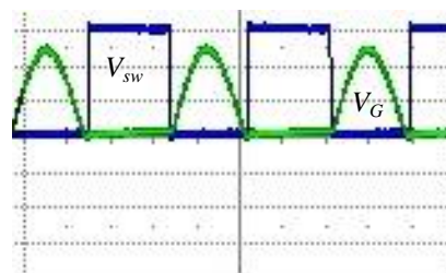
Figure 10.a Control signal , V_{sw} , (20 Volt/div) and voltage at low voltage side , V_G , (5V/div)
