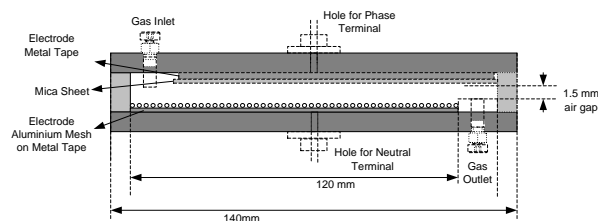
Figure 1. Ozone chamber
