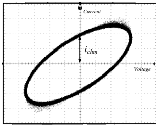
Figure 2. I-V characteristics in Lissajous Pattern
