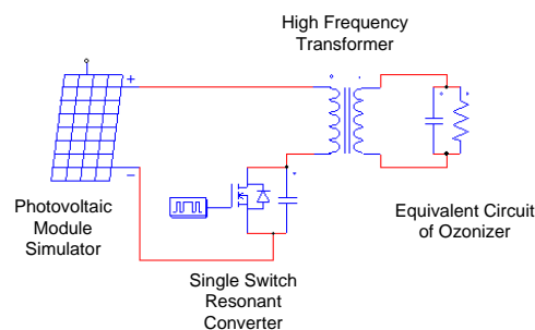
Figure 9. Experimental Set Up of ozonizer for Colour Removal
