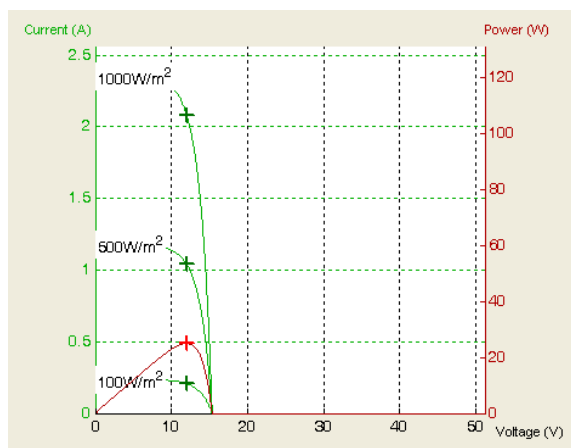
Figure 9. IV Curve of Photovoltaic
