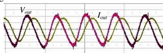
Figure 10.a Output voltage at terminal chamber Voltage (500V/div) and Current (20mA/div) at chamber side
