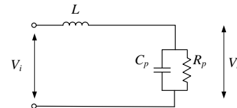
Figure 7. Equivalent Circuit of Ozone Chamber as part of Parallel Loaded Resonant Circuit
