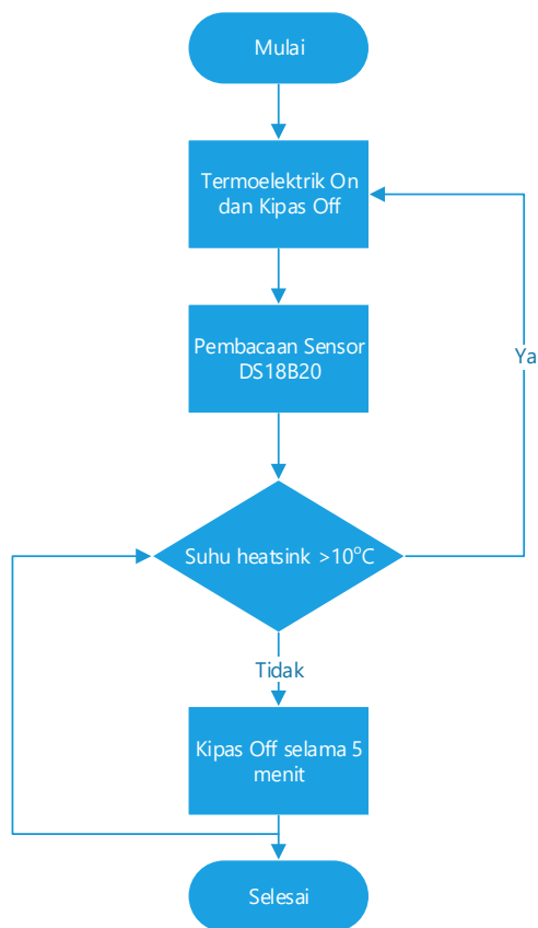
Gambar 5. Flowchart Program
